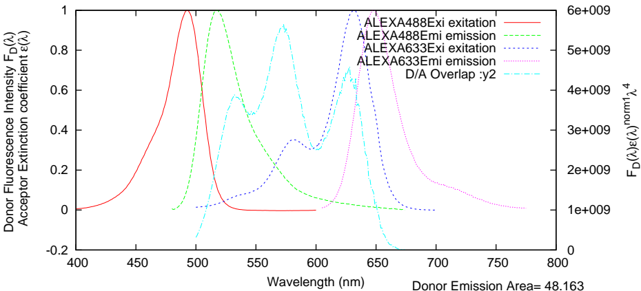
ALEXA488Emi-ALEXA633Exi FRET Donor/Acceptor spectre
